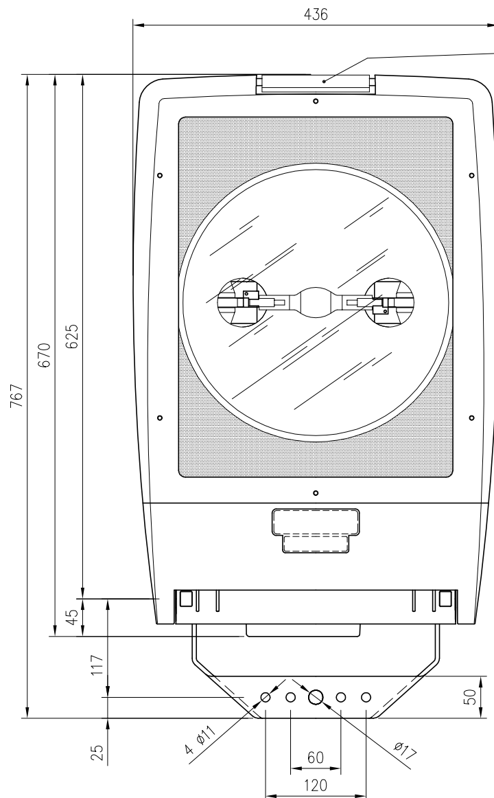
VISTA FRONTAL
