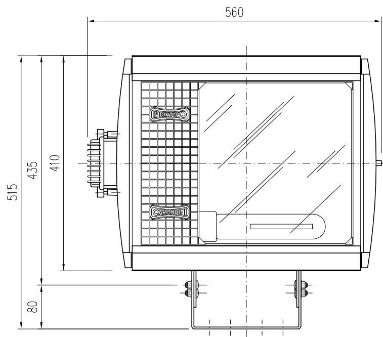
VISTA FRONTAL
