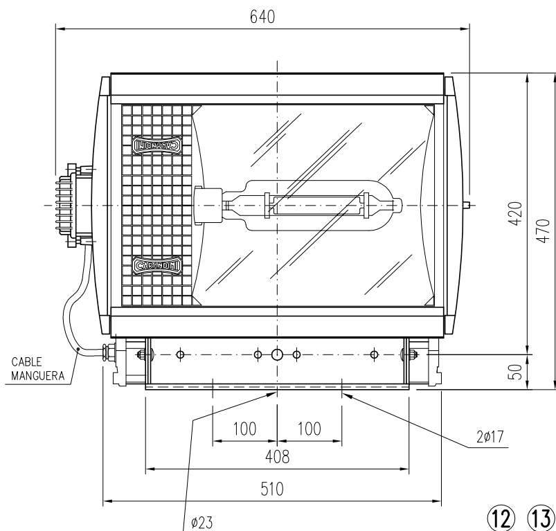
VISTA FRONTAL
