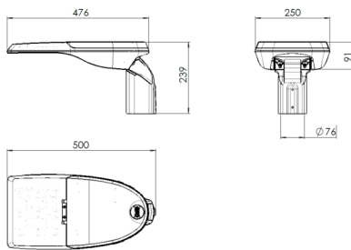
Vertical fixation \varnothing 76 mm (PT1)
